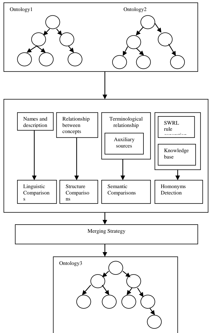
Figure2. Proposed Architecture
