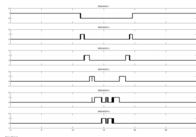
Figure 6.1.A3 Operation of the Breakers
