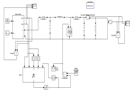
Figure 2.1: MATLAB/Simulink model for MPPT unit LOAD = 100 Ω
