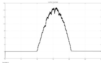
Figure 6.1.A2 Output voltage of MPPT unit
