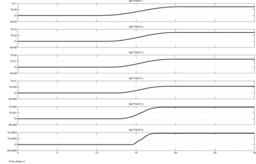
Figure 6.1.A4 SOC of all the batteries in the array
