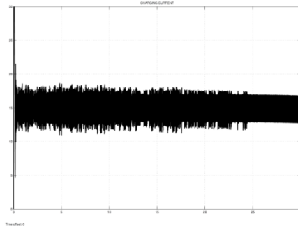
Figure 10.1.1 Charging current For a 12 V, 150 Ah battery, the rated Charging current is 15 A.
