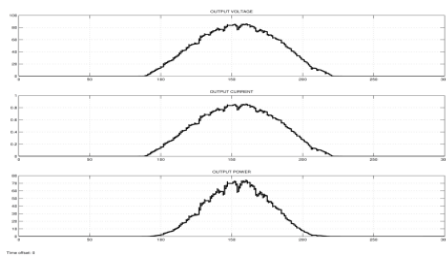
Figure 1.2.4: Output of the solar model with MPPT
