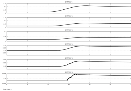
Figure 6.1.A1 Terminal voltage of all the batteries in the array
