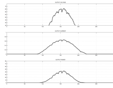
Figure 1.2.3: Output of the solar model without MPPT
