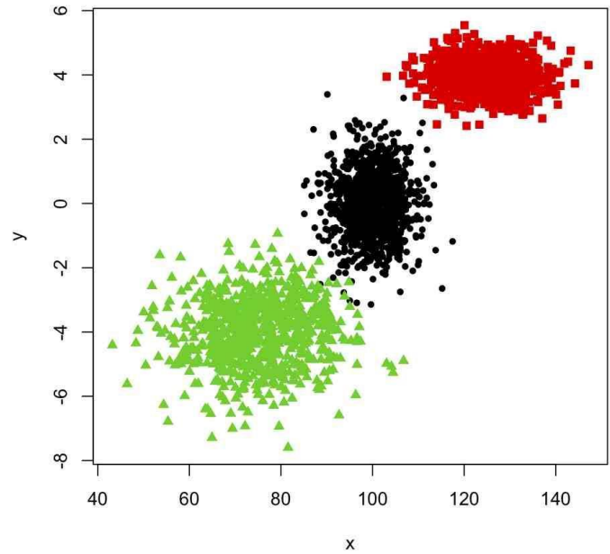
Fig 5: K-Means output
