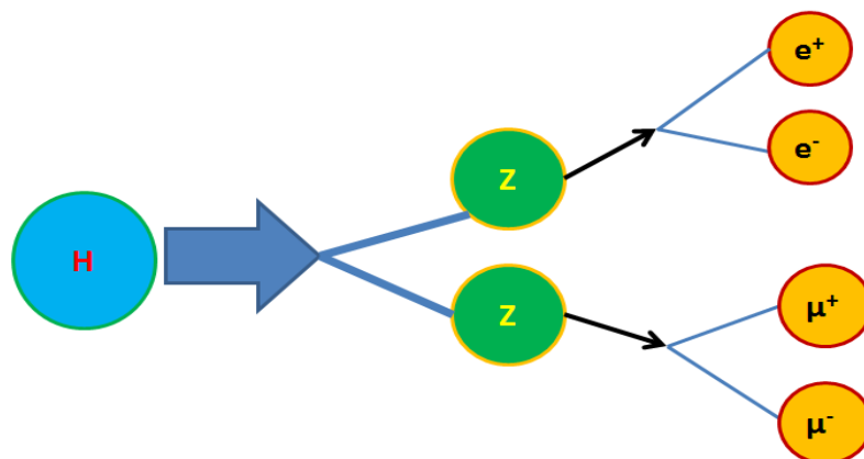
Fig. 16 The Higgs Boson and the Z Bosons decay in a tiny fraction of a second (approximately 10^{-22} seconds) into electrons and muons ( e^+ e^- \mu^+ \mu^- ) with a combined mass of about 125 to 126 GeV .
