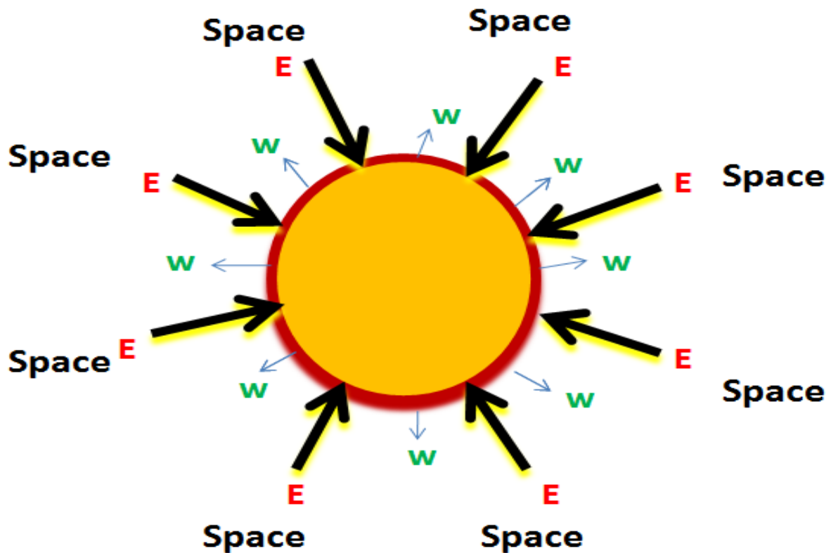
Fig. 1 Downward arrow denotes 'Self-Compressive Surrounding Pressure Force (E)' and upward arrow denotes 'Repulsive Force (w).'
