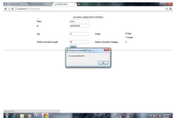
Fig.3 Limit validation
