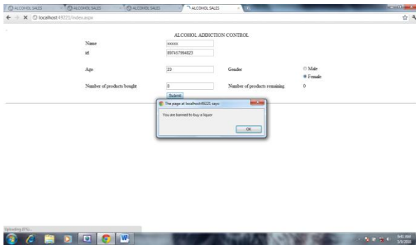
Fig.4. Age validation
