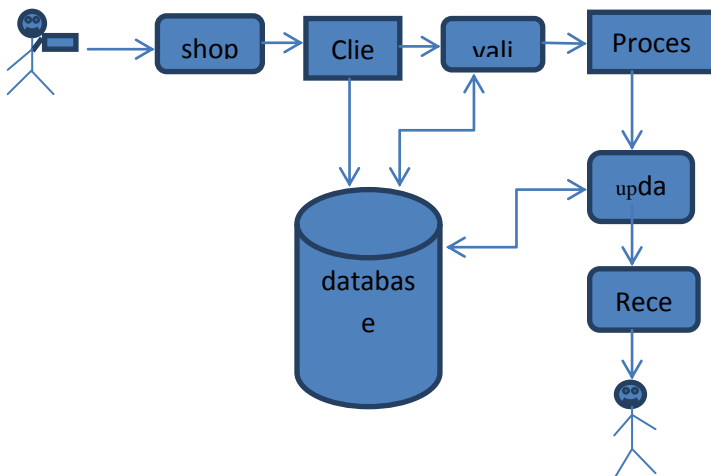
Fig.1. Workflow
