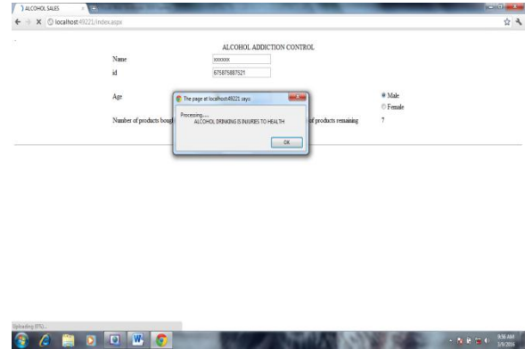
Fig.5 Final Processing
