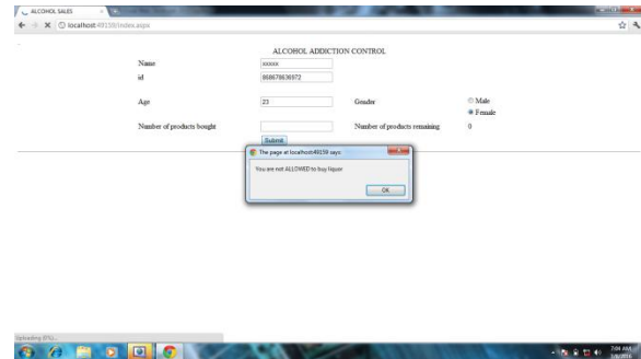
Fig.2. Gender validation
