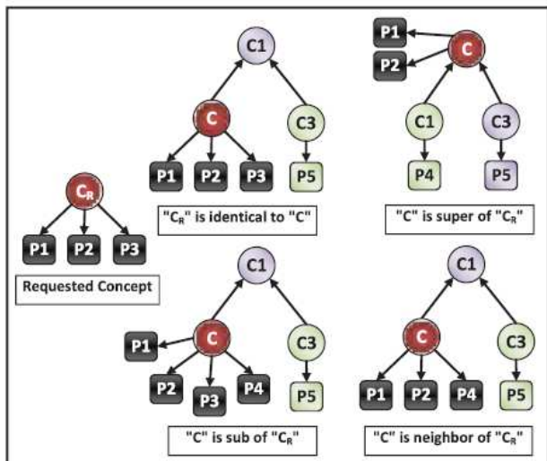
Figure.2. Concept relationships
