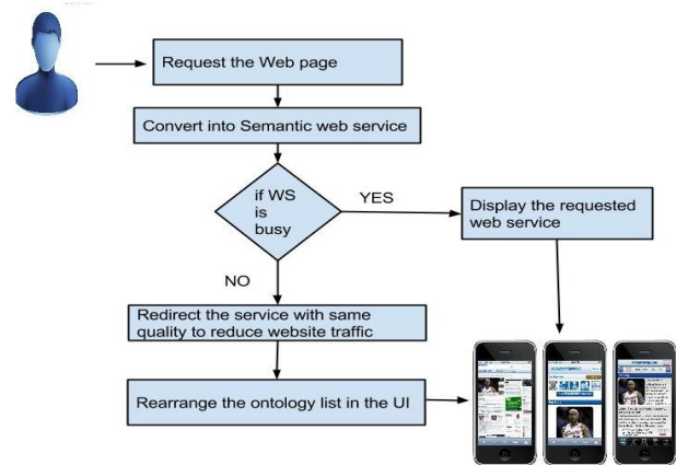
Figure.3. Work flow for ranking mechanism
