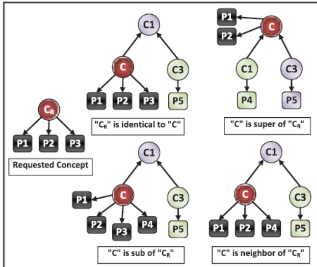
Figure.2. Concept relationships
