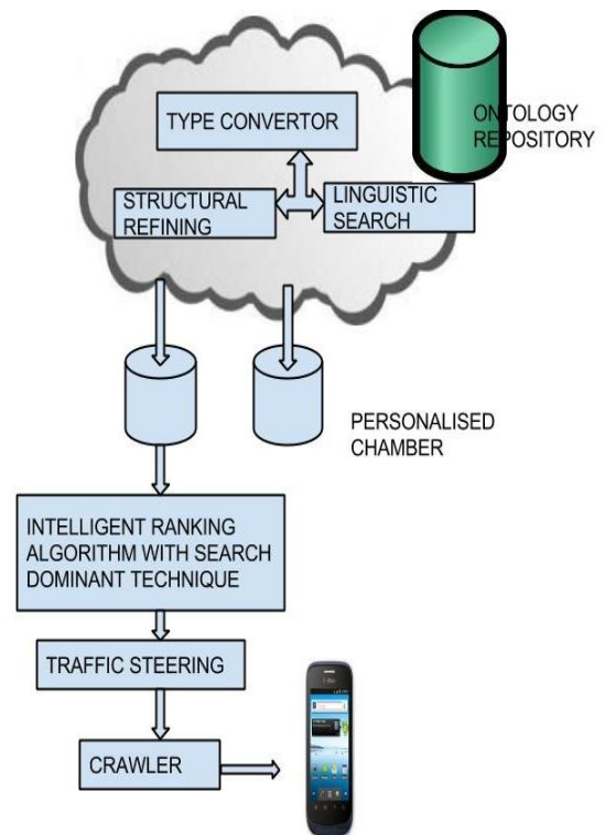
Figure.1. System organisation
