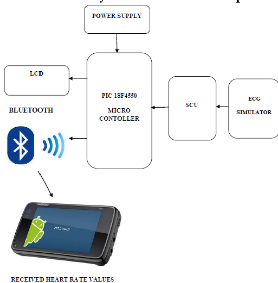
Block diagram of Proposed System
